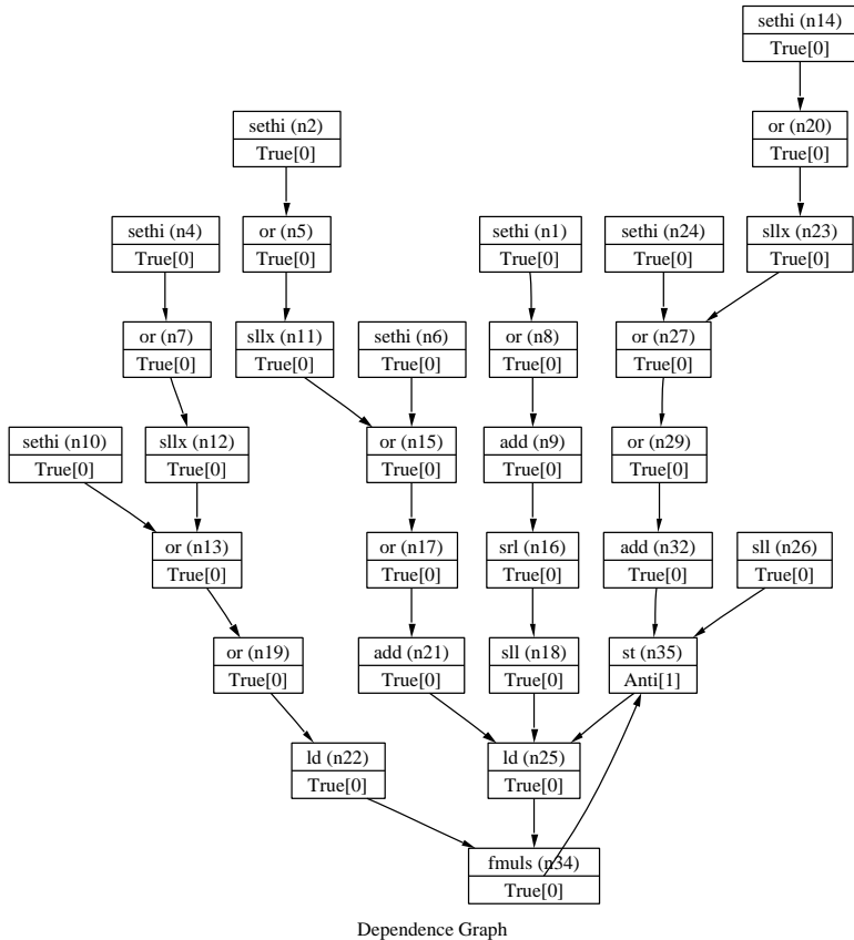
Figure 4.4: Dependence Graph After Dependence Analysis
