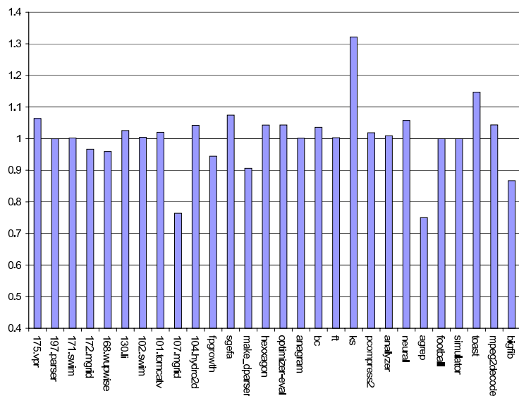
Figure 6.2: Theoretical II to Achieved II Ratio
