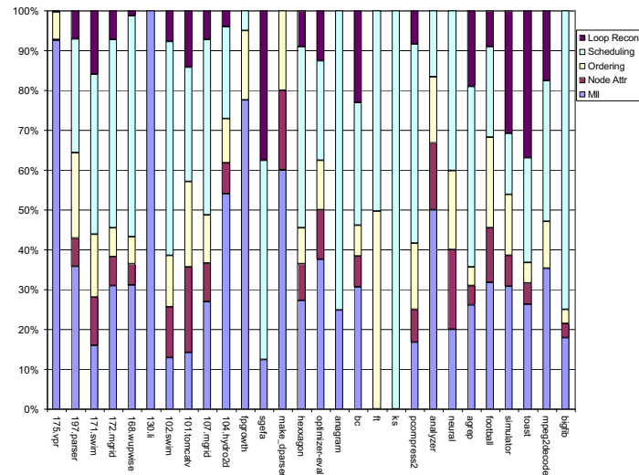
Figure 6.1: Compile Times for the Phases of SMS
