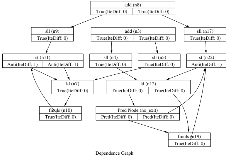
Figure 5.5: Dependence Graph After Dependence Analysis
